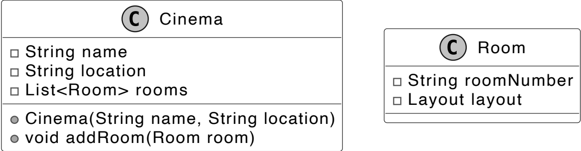
Cinema and Room classes
