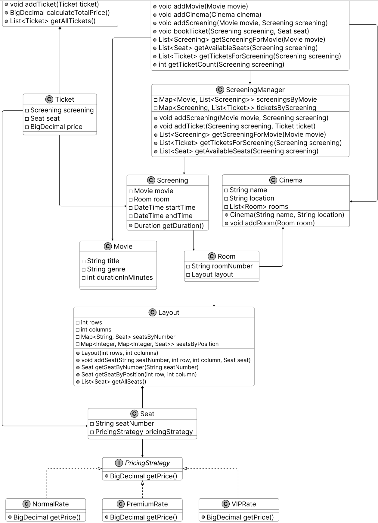
Class Diagram of Movie Ticket Booking System
